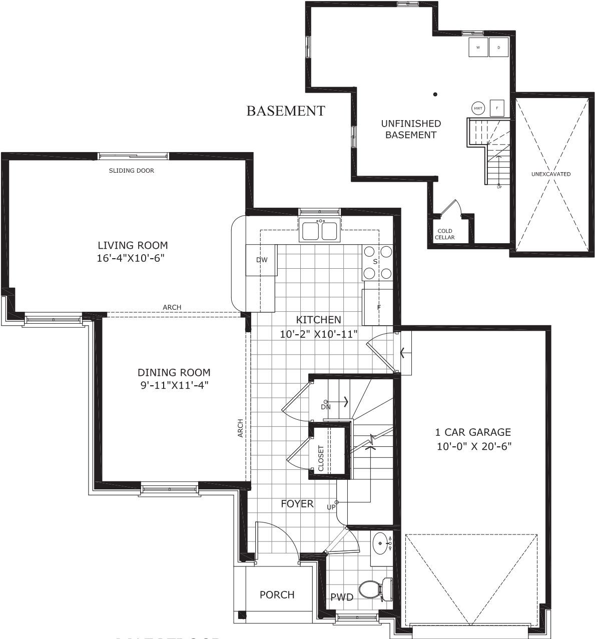
MAIN FLOOR
